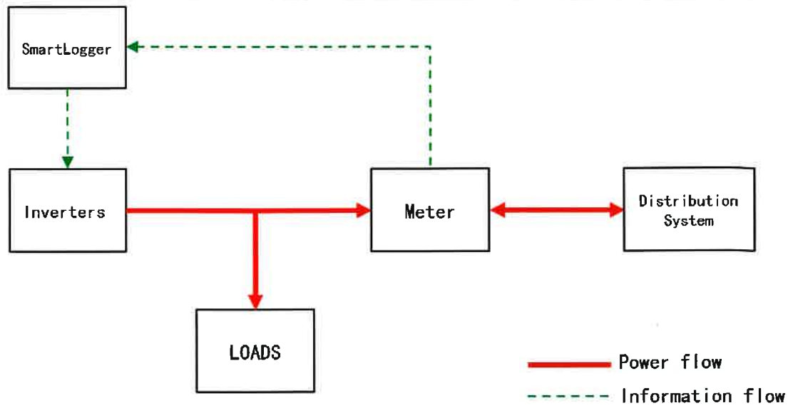
Figure 1. Control Scheme
