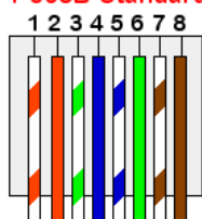
T-568B Standard
