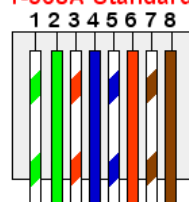
T-568A Standard
