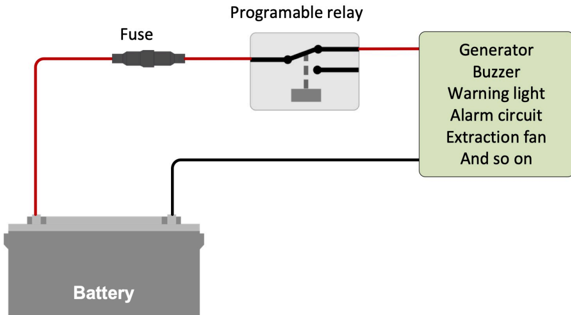
Figure 1. Programmable relay wired to operate a load
