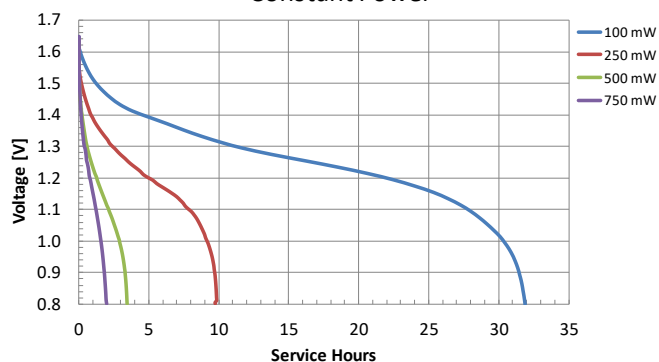
Constant Power
