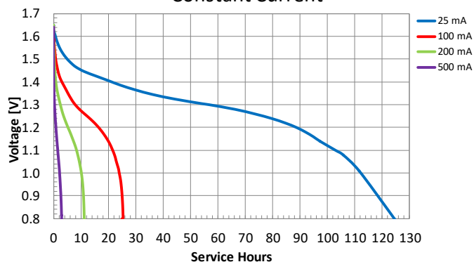
Constant Current
