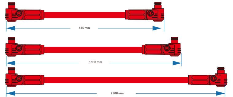
PE cable(1PCS)
