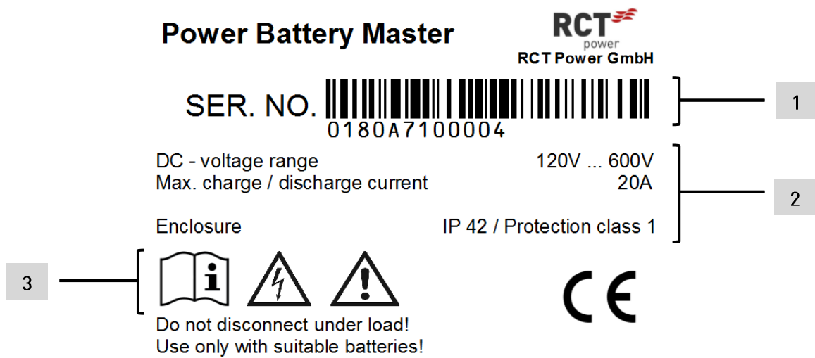
Fig. 3-5 Name plate
