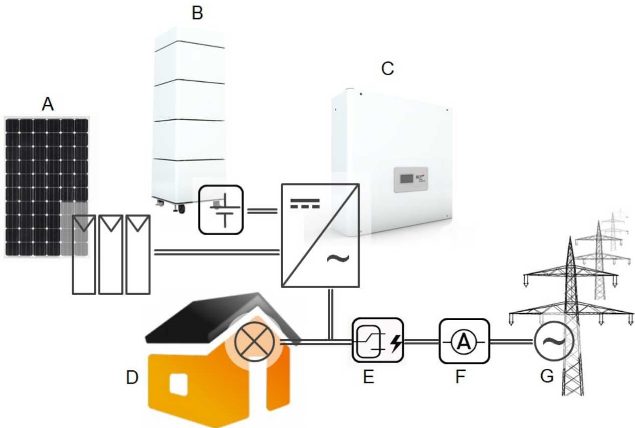
Fig. 3-1 Intended use of the Power Storage and Power Battery in the PV System
